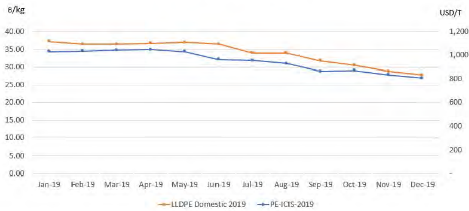
LLDPE ICIS & Domestic Price 2019
